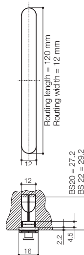
Lockcase routing detail
