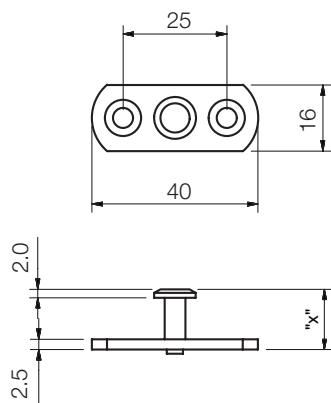
Capture Restrictor LH - Short
