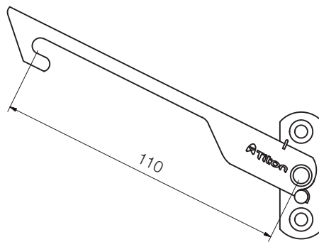
Capture Restrictor LH - Medium
