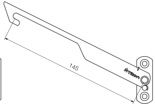
Capture Restrictor LH - Long
