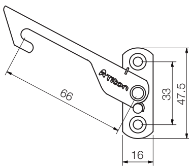
Capture Restrictor LH - Short
