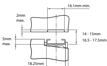
Venture with bottom hinge packer section details
