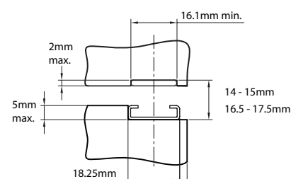
Venture section details
