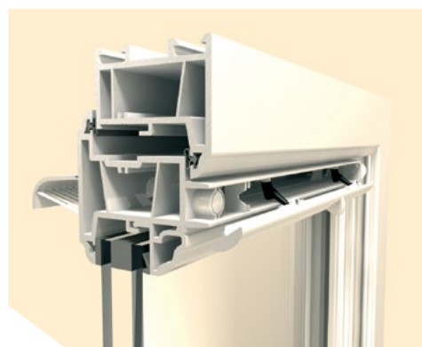
Through sash
